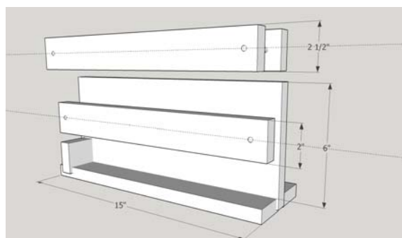
Figure 4. Book Frame/Press The holes mark \frac{1}{4} - \frac{5}{16} " bolts with knobs or wing nuts to tighten the clamp boards against the book block. Varnish and wax the insides of the top clamp or use waxed Melamine
